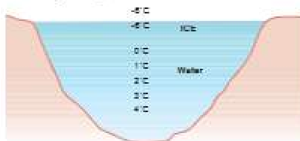
Fig. 11.3 Thermal zones in cold water bodies
