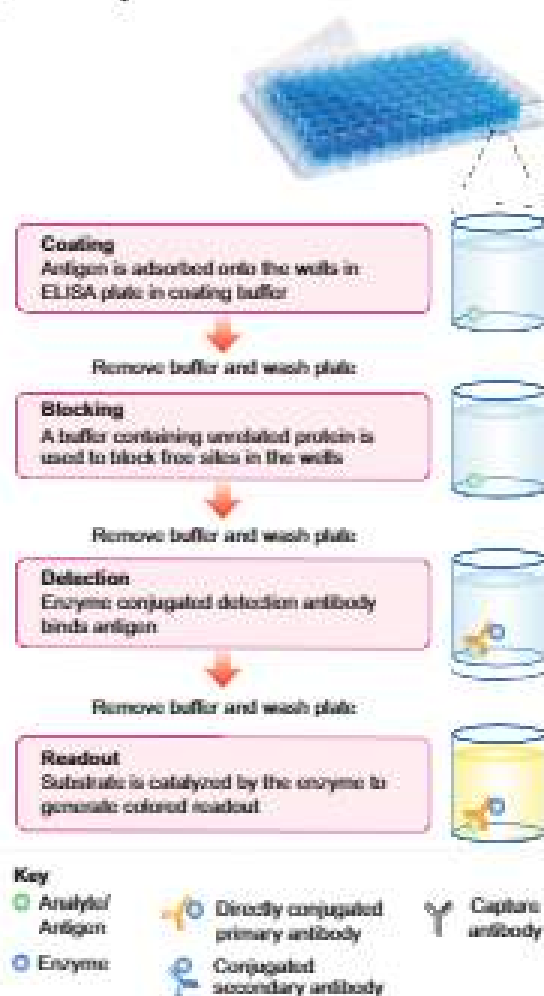
Fig. 10.5 Enzyme Linked Immuno Sorbent Assay
