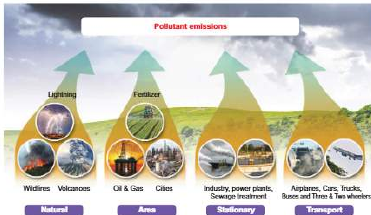
Fig. 13.1 Sources of air pollution.
